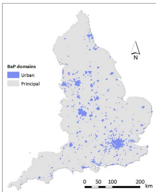
Figure 4: BaP domain map.
