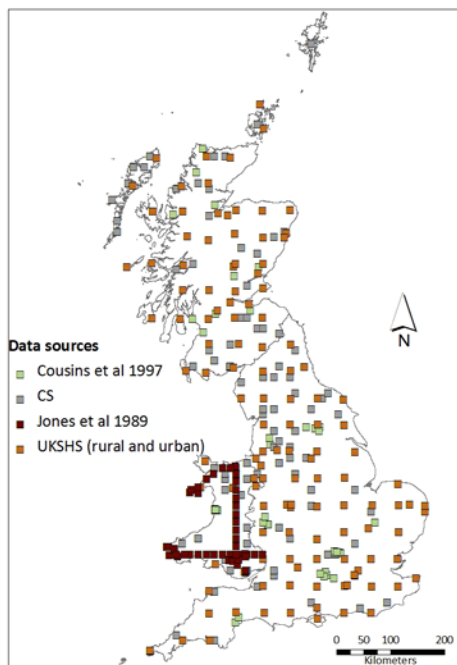
Figure 2: Map showing the distribution of samples used in the BaP NBC determination. For references to peer-reviewed data see supplementary information.
