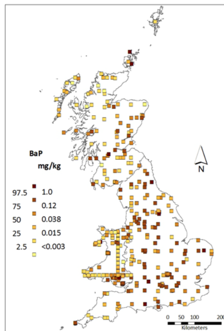
Figure 3: BaP in topsoil as a percentile classified map.
