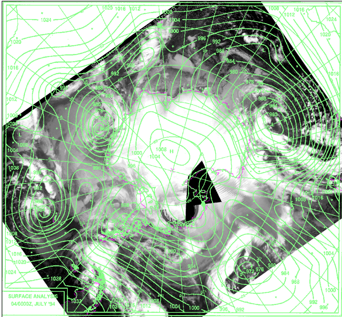
Figure 1.1 Composite of geostationary and polar orbiting infra-red satellite imagery for the nominal time of 0000 UTC 4 July 1994. (The imagery is courtesy of the University of Wisconsin–Madison’s Space Science and Engineering Center. The analysis overlay was produced during the First Regional Observing Study of (the Antarctic) Troposphere Project.)
