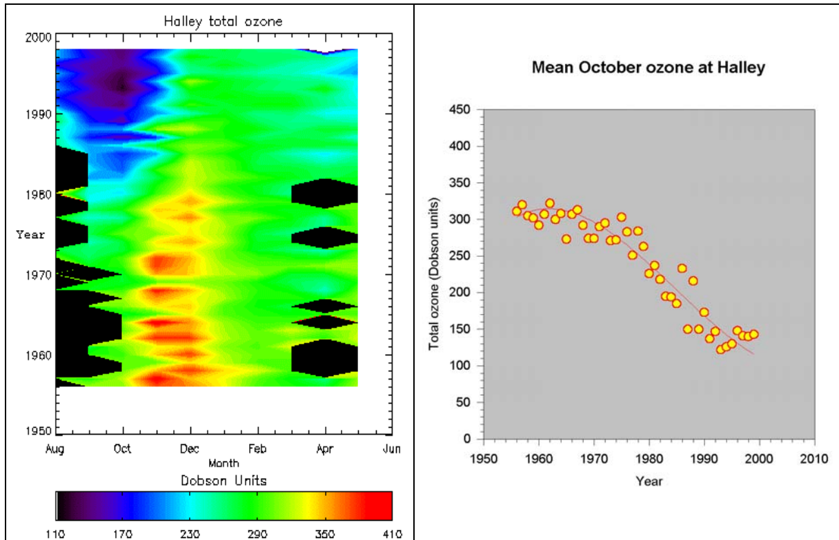
Figure 2.7.2.1 The seasonal variation of total ozone at Halley for the period 1957–98.
