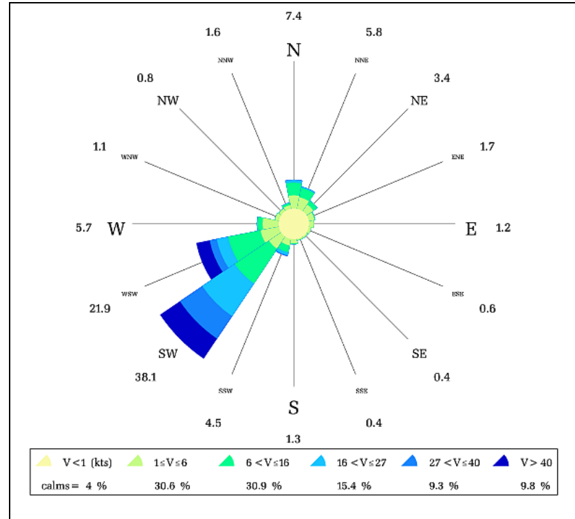
Figure 7.12.2.4.11 Annual-mean wind rose AWS 7358.
