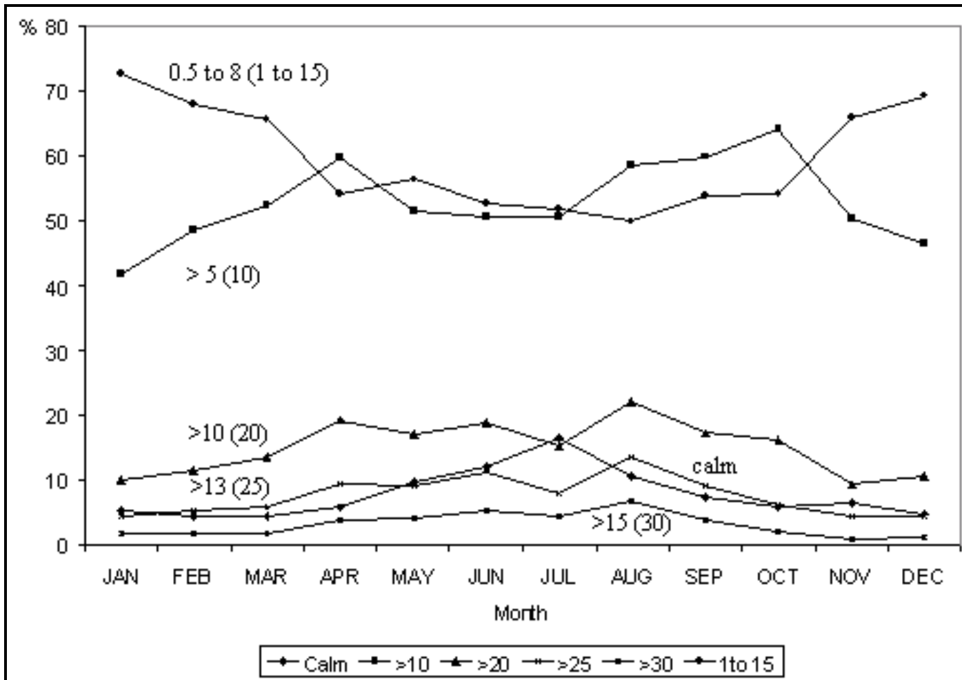
Figure 7.3.2.4.1 Frequency of occurrence of wind speeds higher than certain specified values at Frei Station (~62° 25' S, ~58° 53' W, ~10 m AMSL), King George Island. (The key shows the units in kt while the figure shows m s^{-1} (kt).)
