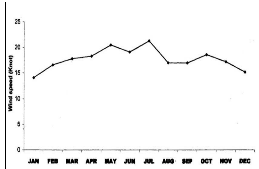
Figure 7.5.7.4.2 Mean–monthly wind speed at Maitri Station ( \sim 70^{\circ} 45' 52'' S, \sim 11^{\circ} 44' 03'' E, \sim 117 m AMSL), Dronning Maud Land, for the period 1990–97.
