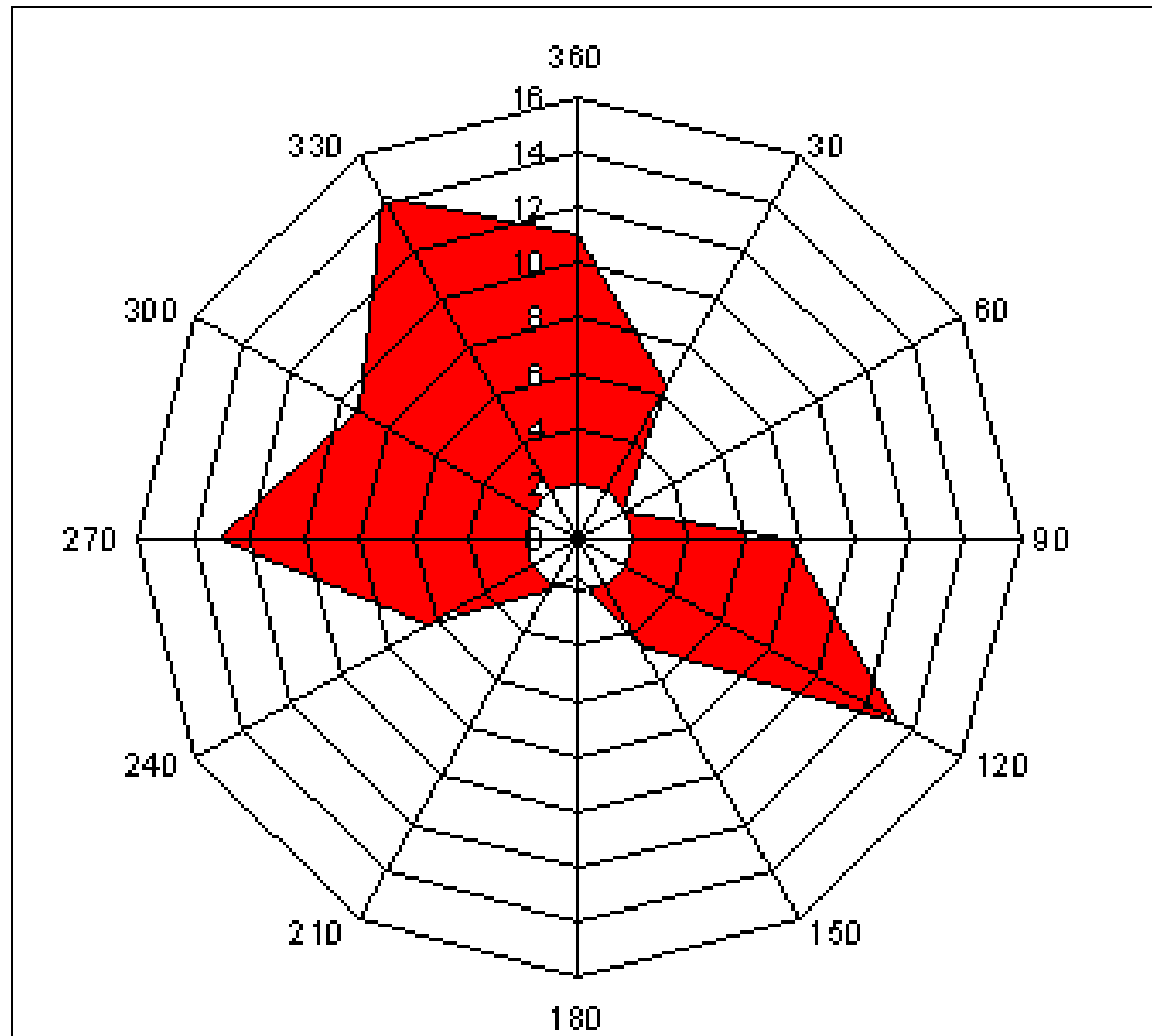
Figure 7.3.2.4.2 Annual mean wind direction at Frei Station ( \sim 62^{\circ} 25' S , \sim 58^{\circ} 53' W , \sim 10 m AMSL), King George Island. (The red area shows the envelope of wind directions at Frei.)
