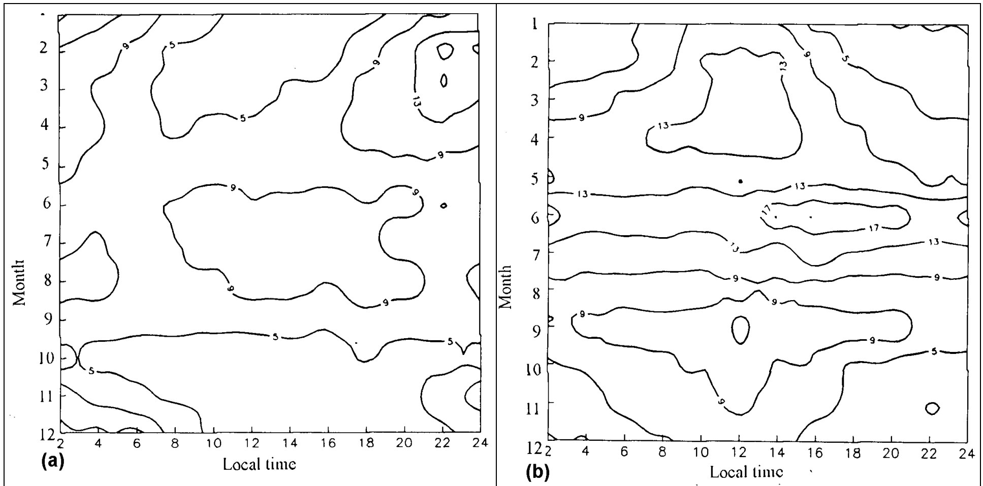
Figure 7.8.3.4.5 (a) Percentage frequency of calms and (b) strong winds-gales at Zhongshan Station ( 69^{\circ} 22' S , 76^{\circ} 22' E , 15 m AMSL), Princess Elizabeth Land, on a monthly (1=January, 12=December) versus local time (hr).
