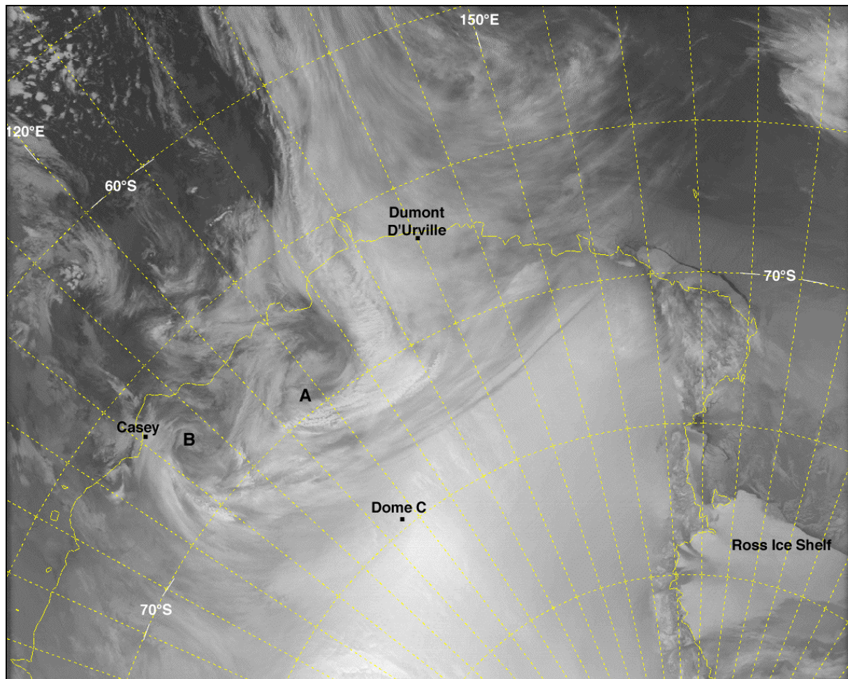
Figure 2.4.6.3.1 A DMSP image of cyclonic vortices over East Antarctica at approximately 2300 UTC 26 July 1994. (From Pook and Cowled (1999) – their Fig. 7a.)
