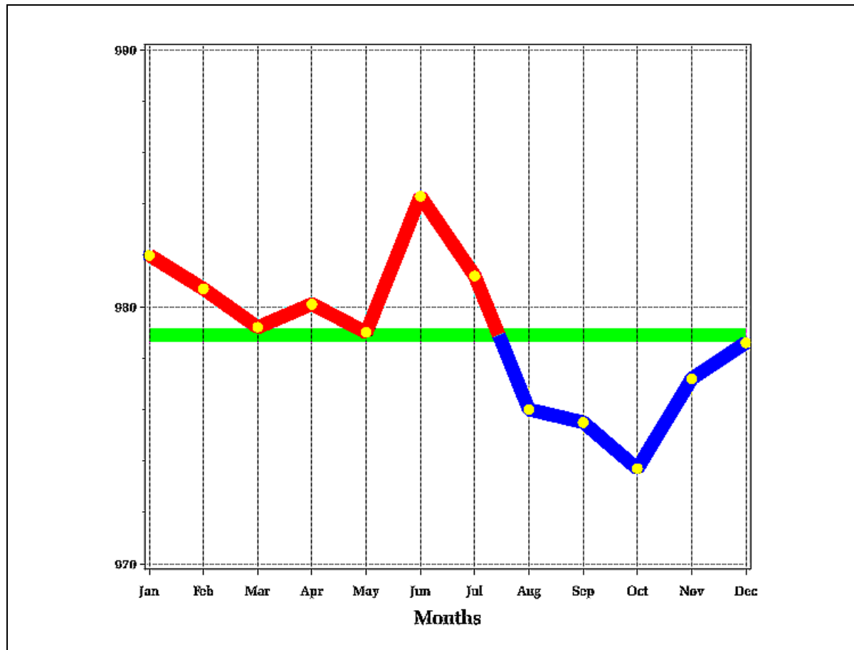
Figure 7.12.2.4.3 Monthly-mean pressure (hPa) for Terra Nova Bay, ( 74^{\circ} 41' 42'' S, 164^{\circ} 7' 23'' E, 17 m AMSL), Victoria Land.
