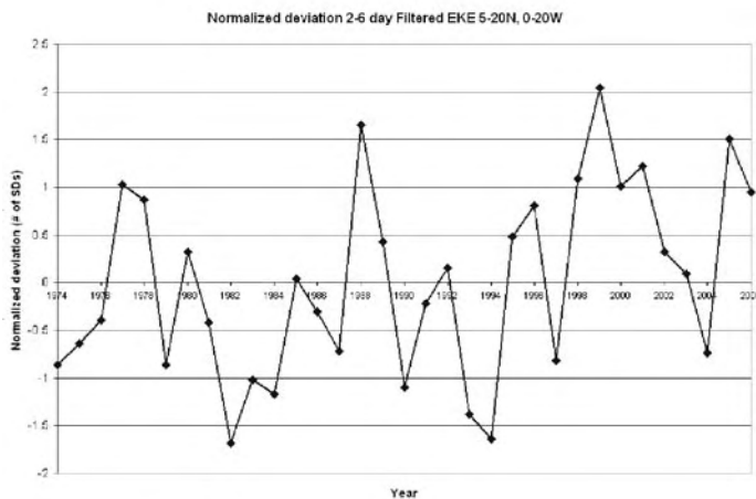
Figure 2 Normalized deviation of 2-6 day filtered eddy kinetic energy, averaged over the region between 5-20N and 0-20W.
