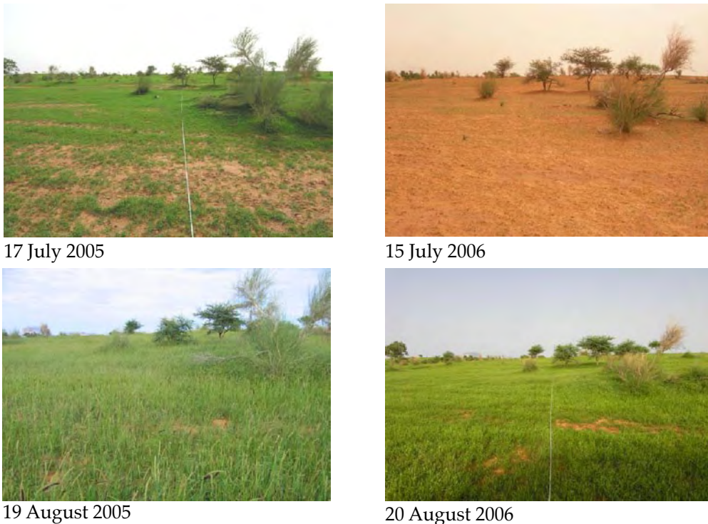
Figure 2 Contrasting vegetation conditions at the Agoufou field site during July and August 2005 and 2006 (courtesy E. Mougin).
