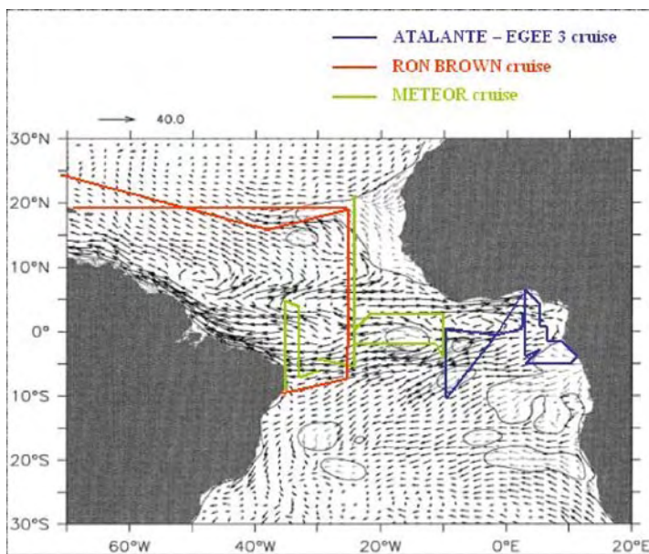
Figure 4. SOP monsoon onset cruise tracks.
