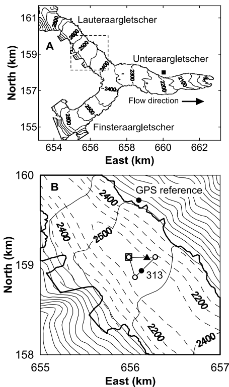
Figure 1. (A) Map of Unteraargletscher and its tributaries. The solid square is the precipitation measurement site. (B) The study area on Lauteraargletscher (smaller square in (A)). Solid and broken contour lines indicate the surface and bed topography, respectively. Elevations are in meters above sea level. Solid circles are positions of a pair of GPS antennas for continuous measurement of surface flow. Open circles connected with solid lines are the strain array, the open square is the location of the boreholes, and the solid triangle is the location of the water pressure measurements. Coordinates correspond to the official Swiss coordinate system.
