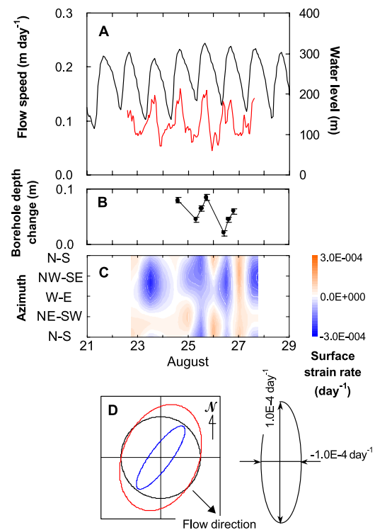
Figure 4. (A) Surface flow speed (red) and borehole water level. (B), Changes in the 173-m borehole depth. (C), Horizontal strain rate on the surface. Strain rates were measured twice a day at 0:00 and 12:00, and the contours estimated by linear interpolation along the time axis. (D), Mean strain rate ellipses of horizontal deformation in the daytime and at night during late August 2001. These represent the original state (black), after the deformation from 6:00 to 18:00 (blue) and that from 18:00 to 6:00 (red) in magnified forms by a factor of 5 \times 10^3 . On the right side in (D) is a scale that shows 10 -4 day -1 of tensile strain rate in N-S and the equivalent compression in W-S.
