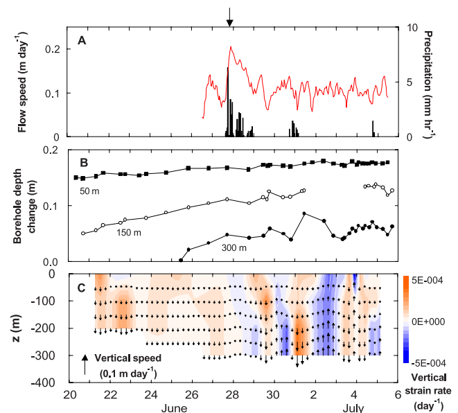
Figure 2. (A) Surface flow speed (red) and hourly precipitation rate. (B) Borehole depth changes in the 50-m (solid square), 150-m (open circle), and 300-m (solid circle) boreholes. (C) Depth distribution of vertical flow speed and vertical strain rate (right side) during late June and early July 2001. Ticks on the temporal axes indicate 0:00 local time. The arrow in (A) shows the motion event described in the text. In (B), measurements in the 150-m borehole were interrupted 1–4 July because snow temporarily clogged in the borehole. In (C), z -axis is pointing upward from the origin at the glacier surface.
