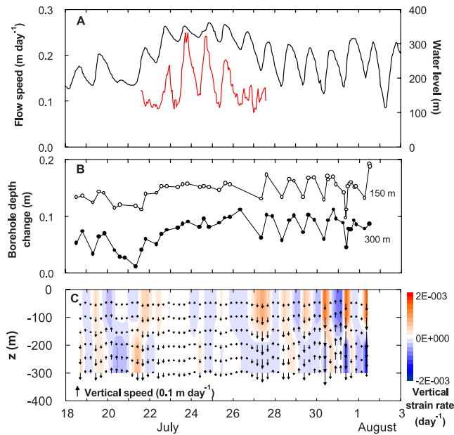
Figure 3. (A) Surface flow speed (red) and water level in the bottom-reaching borehole measured from the glacier bed (black). (B) Borehole depth changes in the 150-m (open circle), and 300-m (solid circle) boreholes. (C) Depth distribution of vertical flow speed and vertical strain rate (right side) during late July 2001.
