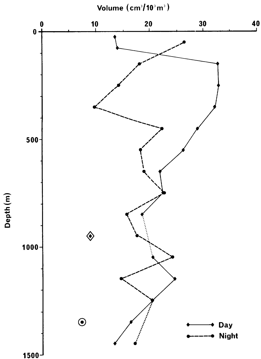
Figure 2. Day and night profiles of displacement volume for RMT1M <4.5mm plankton samples in top 1500m of water column, normalised to 10^3 \text{ m}^3 of water filtered.
