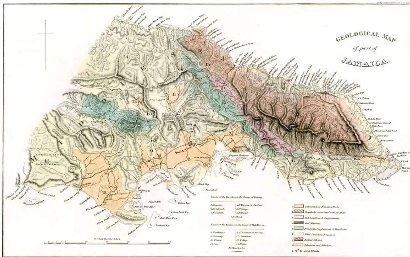
Figure 9. Geological map of the eastern part of Jamaica, surveyed by De la Beche in 1824 (from Transactions of the Geological Society , 1827).
