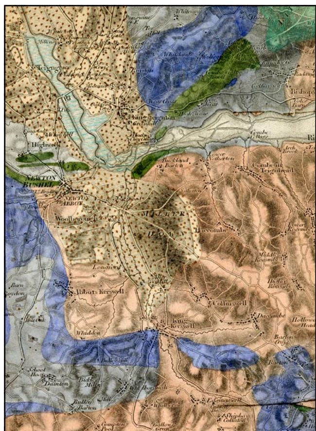
Figure 11. Detail (Newton Bushel) from old series one inch geological sheet 22, south-east Devon, surveyed 1830-31, published 1834: the first Geological Survey map to be submitted for engraving (from De la Beche's own copy, BGS Library AM 1112 S, set A).
